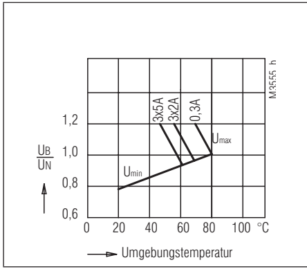
Operating voltage limit curve OA 5621
