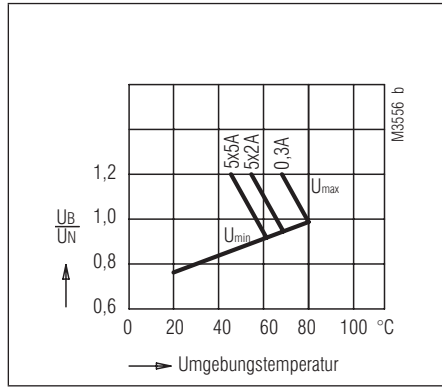
Operating voltage limit curve OA 5622
