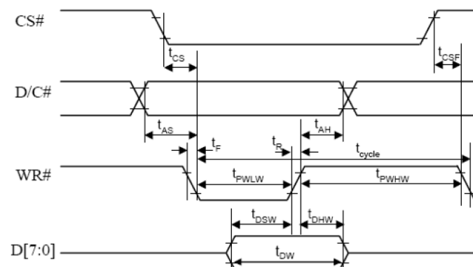
Write Timing
