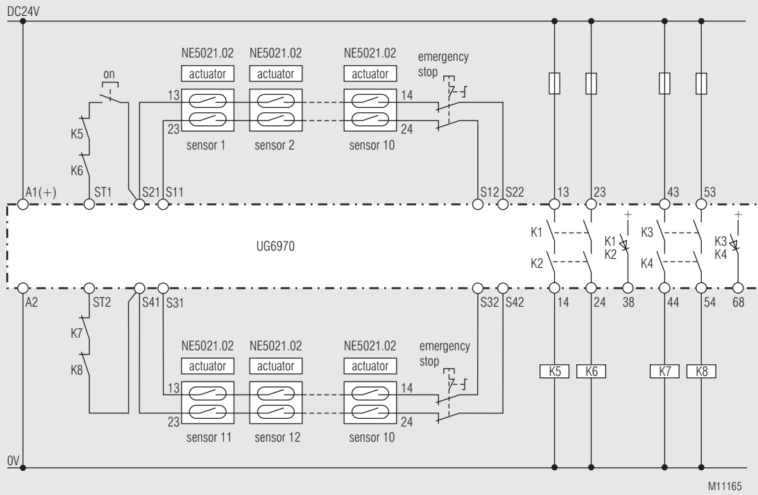
Safety function each 10 magnetic switches NE 5021 +1 E-stop button in series on multifunction safety relay UG6970 Operation mode: 2 (Fkt1 = MANUAL ; Fkt2 = AUTO) Safety function 1: E-stop with cross fault detection (1) , Manual-Start Safety function 2: E-stop with cross fault detection (1) , Auto-Start
