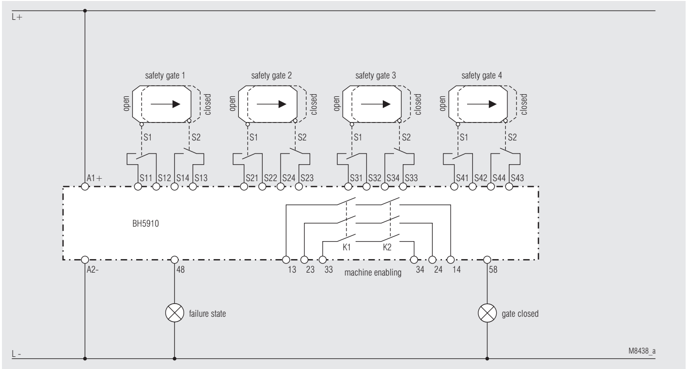
Pic. 8: Gate monitor, 4 gates with 2 NO gate contacts each (switch 1 in position 3; switch 10 in position 0)
