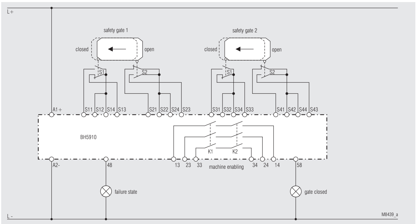
Pic. 9: Gate monitor, 2 gates with 2 changeover gate contacts each (switch 1 in position 3; switch 10 in position 2)
