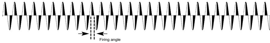
Output with Phase angle switching mode @ 50% input level:
