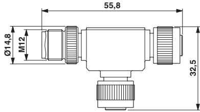
Dimensioned drawing
