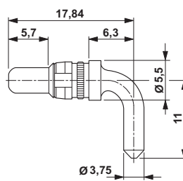
Dimensional drawing
