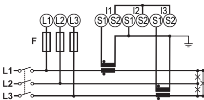
Fig. 9 Three-phase system without neutral (3-wire) unbalanced load and 2 CT (Aron). 315 mA fuse (F).
