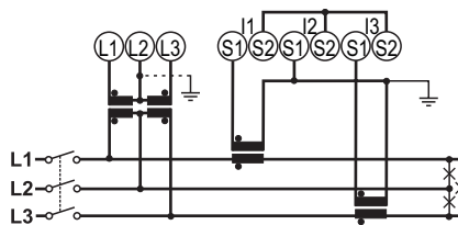
Fig. 10 Three-phase system without neutral (3-wire), unbalanced load, 2 CT (Aron) and 2 VT/PT.
