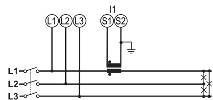
Fig. 11 Three-phase system without neutral (3-wire), balanced load, 1 CT.
