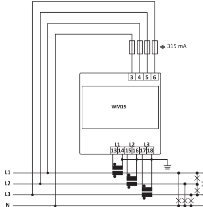
Fig. 11 Three-phase with neutral (4-wire)
