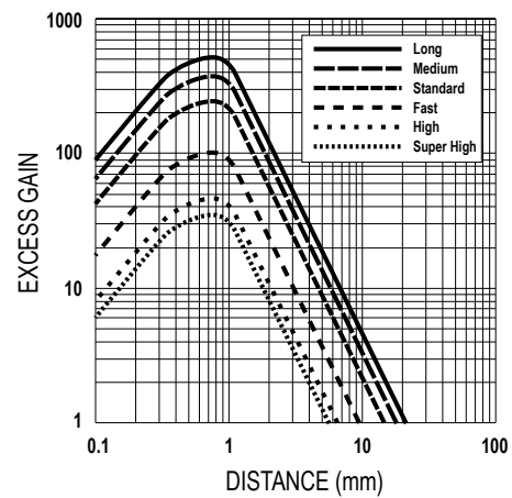
Diffuse proximity with 0.2 mm internal fiber optic diameter
