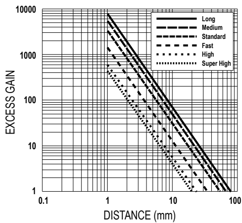
Through beam with 0.2 mm internal fiber optic diameter
