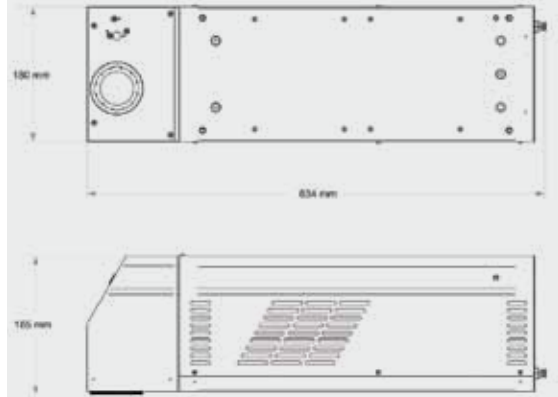
RESONATOR
