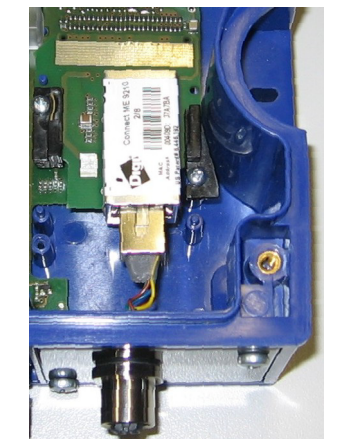
Figure 6 – Ethernet TCP/IP Module – IP65 Mounting
