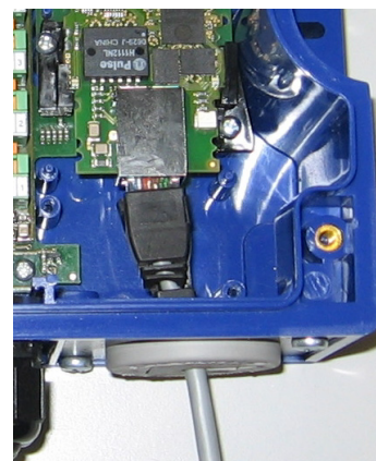
Figure 7 – Ethernet/IP Module IP54 Mounting
