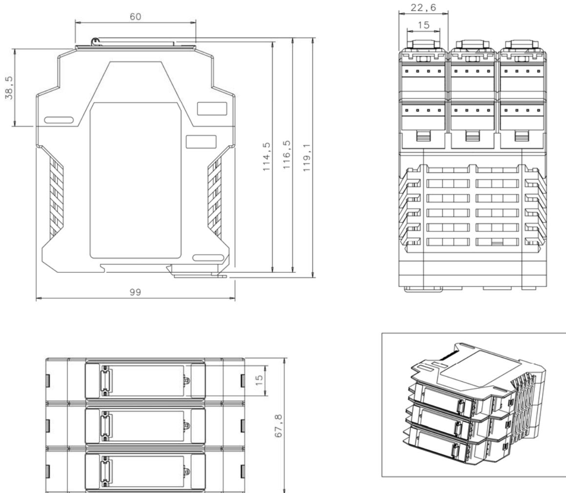
Fig. 37 SG-BWS-T4-MT overall dimensions
