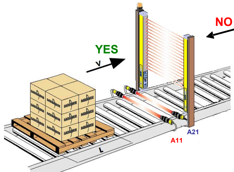
Fig. 31 Uni-directional muting
