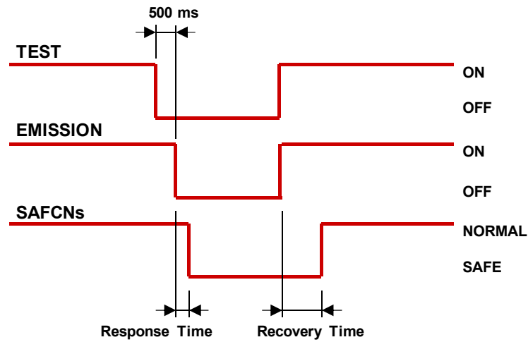
Fig. 25 Test function timings
