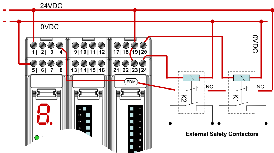
Fig. 21 EDM connections
