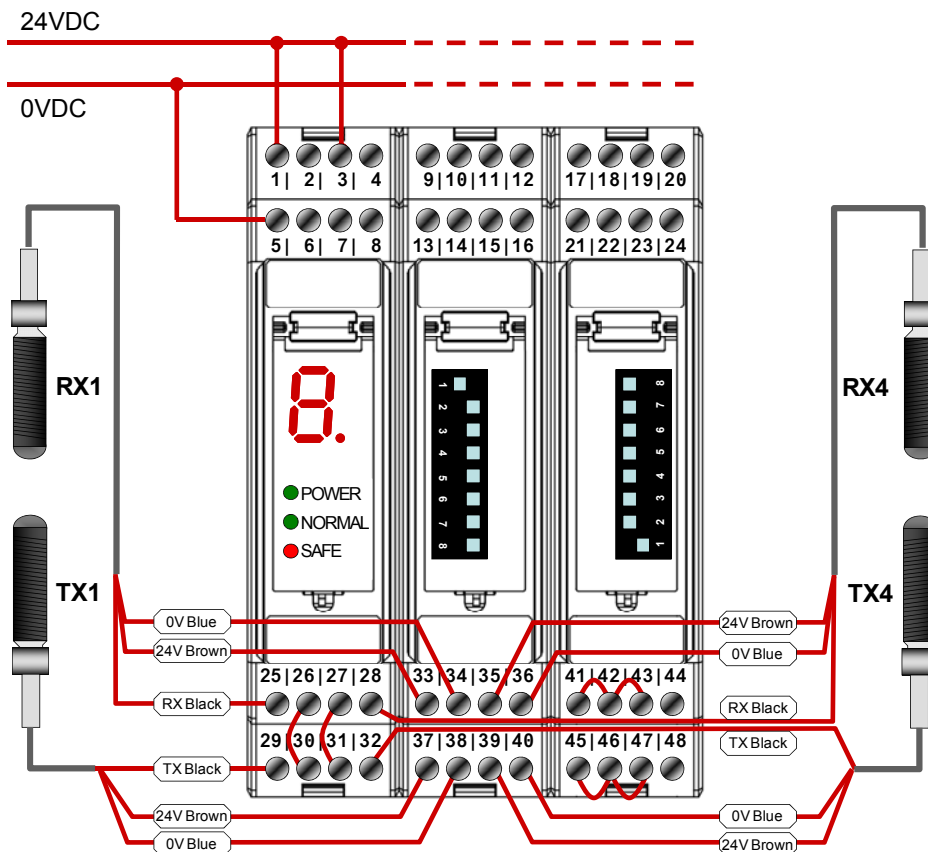
Fig. 20 Safety photocells connection
