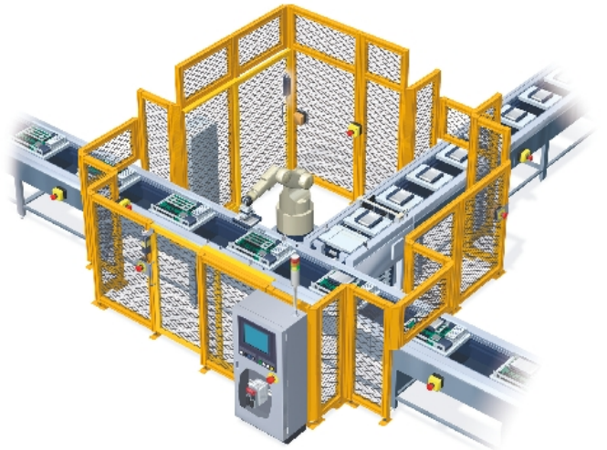
Fig. 5 Conveyor protections
