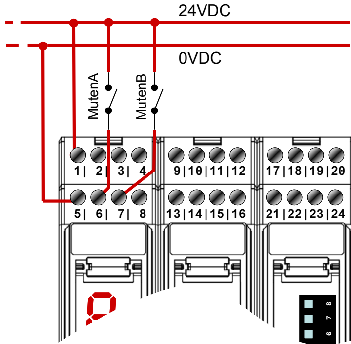
Fig. 26 Muting enabling switches connection
