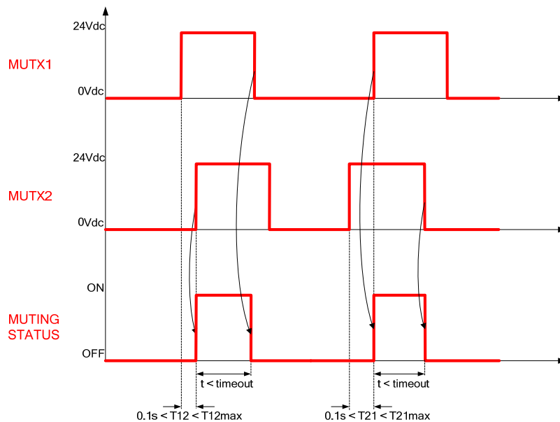
Fig. 35 timings muting T
