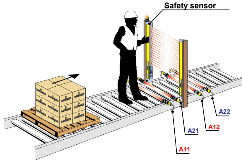
Fig. 28 Muting: typical application
