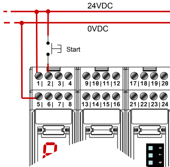
Fig. 23 Start button connection
