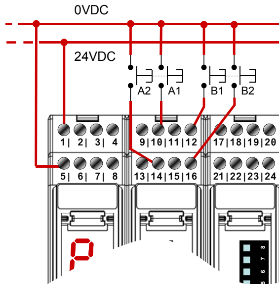
Fig. 36 Override switches connections
