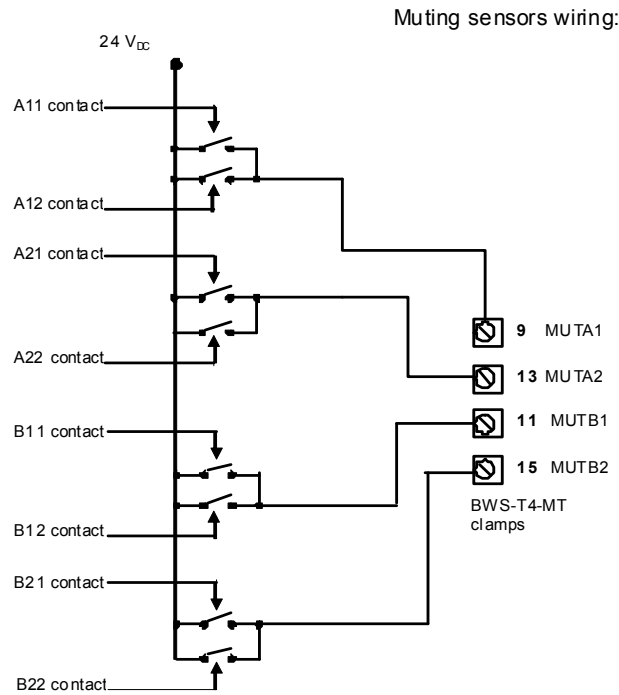
Fig. 30 Muting: 8 sensors application connections
