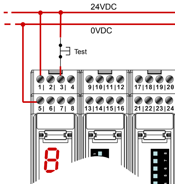
Fig. 24 Test/Reset switch connection
