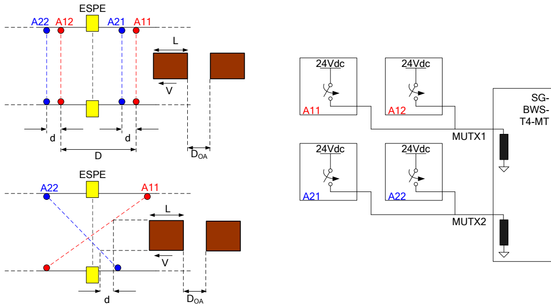
Fig. 34 muting T connection
