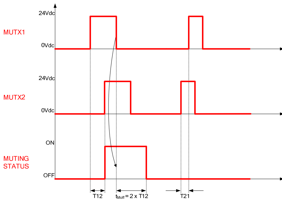
Fig. 33 muting L timings
