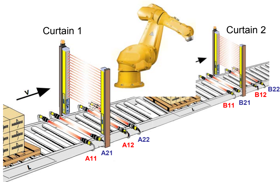
Fig. 29 Muting: 8 sensors application
