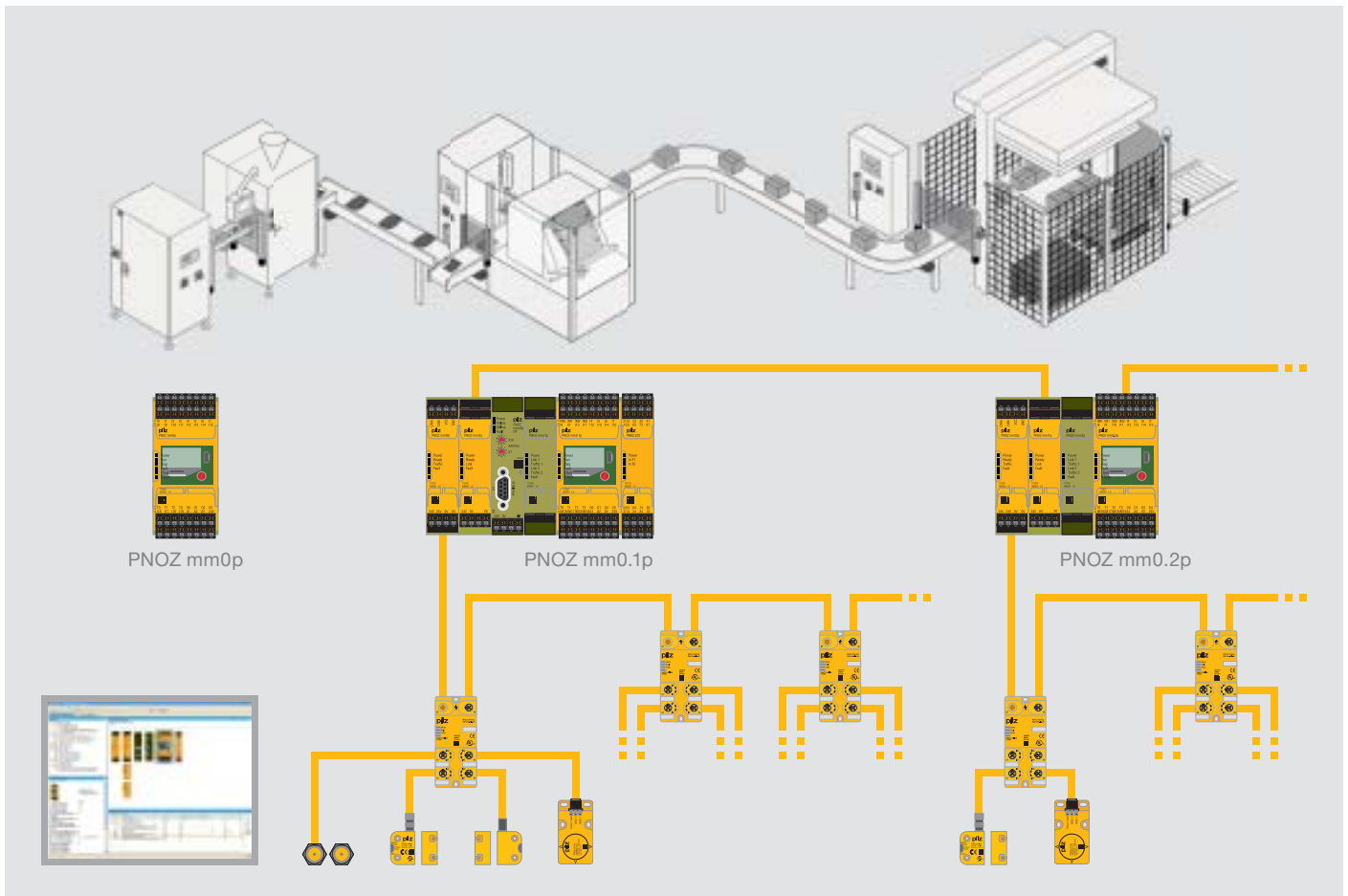
PNOZ mm0.1p
