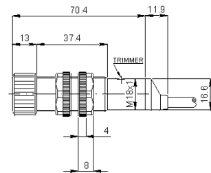
M12 CONNECTOR
