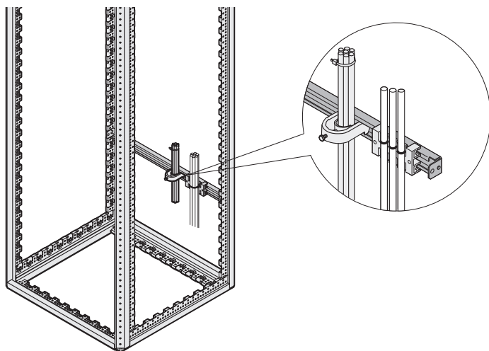
C-profile
