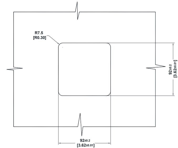
Panel Cutout
