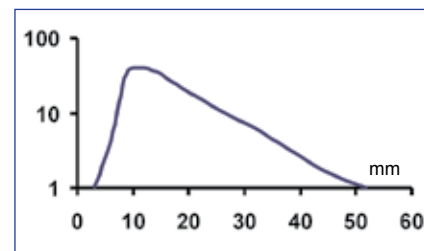
Fixed focus proximity - 50 mm - Excess gain
