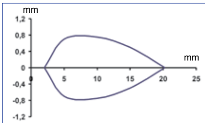
Fixed focus proximity - 20 mm - Detection area
