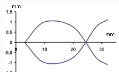
Fixed focus proximity - 30 mm - Detection area
