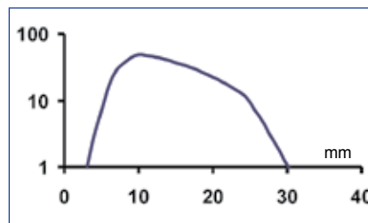
Fixed focus proximity - 30 mm - Excess gain
