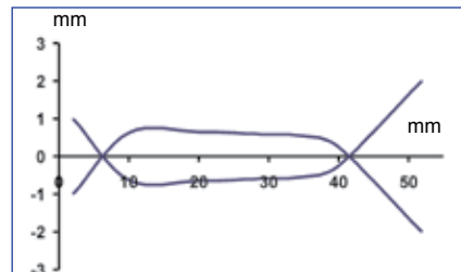
Fixed focus proximity - 50 mm - Detection area
